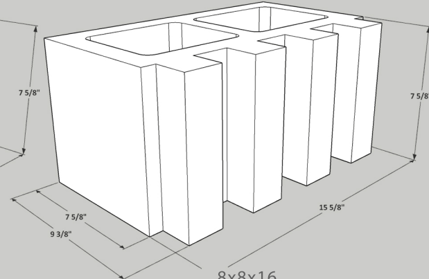
8x8x16 Fluted Block
