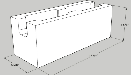
6x6x16 Bond Beam Block
