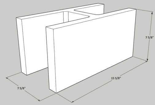
8x8x16 Double Open End Block
