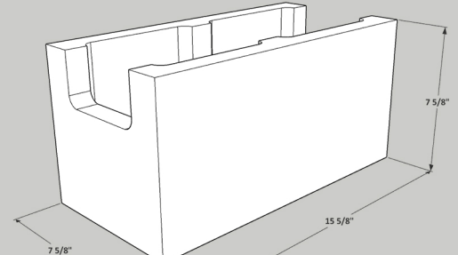
8x8x16 Bond Beam Block
