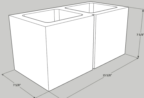
8x8x16 Single Score Block
