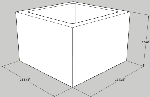
12x8x12 "O" Block
