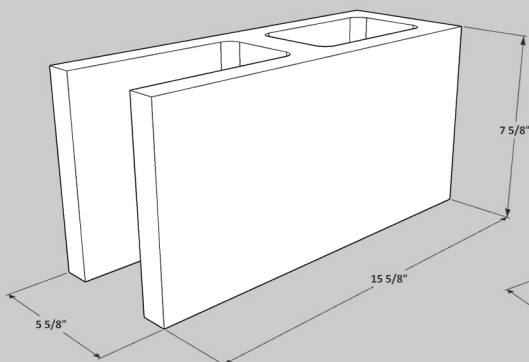
6x8x16 Single Open End Block
