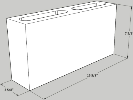
4x8x16 Partition Block
