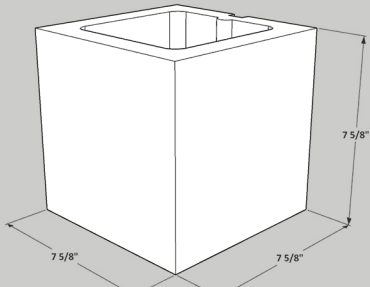
8x8x8 Half Block
