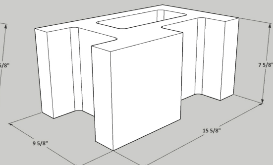
10x8x16 L Block
