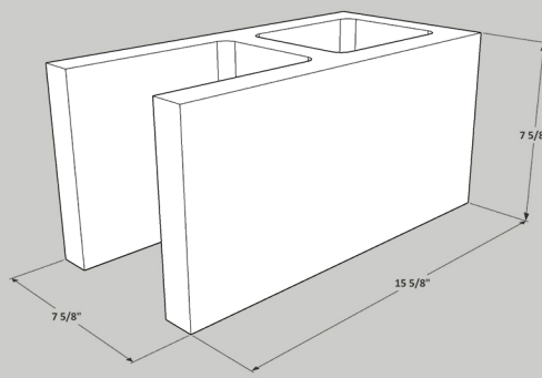
8x8x16 Single Open End Block
