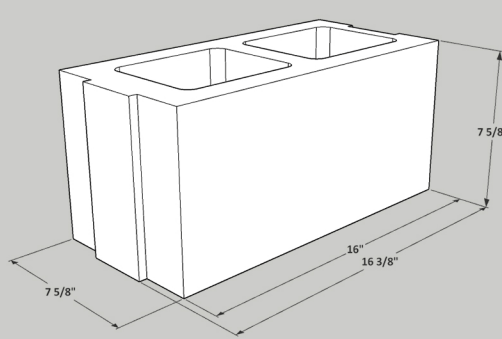
8x8x16 Interlock Block
