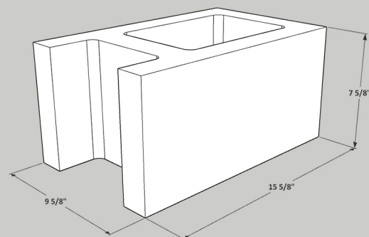
10x8x16 A Block
