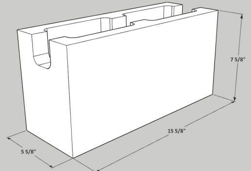
6x8x16 Bond Beam Block
