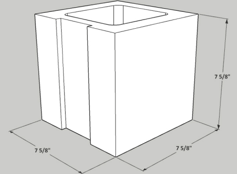
8x8x16 Interlock Half Female Block
