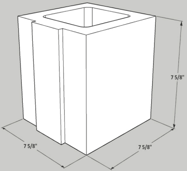
8x8x8 Interlock Half Male Block
