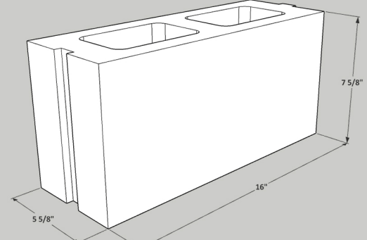
6x8x16 Interlock Block
