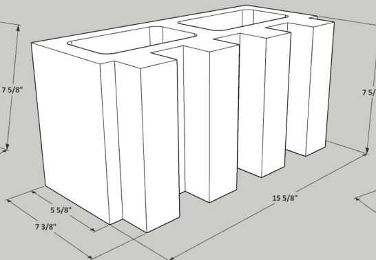
6x8x16 Fluted Block
