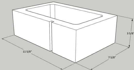
12x4x8 Half Block
