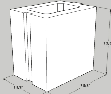
6x8x8 Interlock Block
