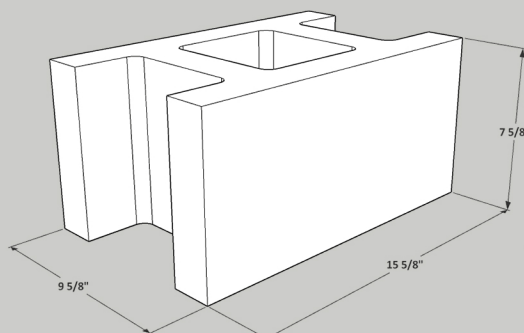
10x8x16 H Block
