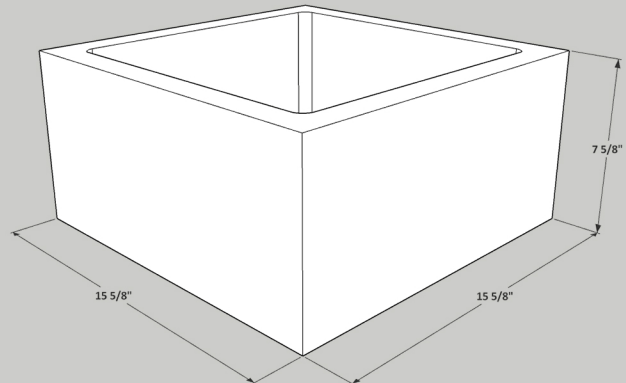
16x8x16 "O" Block
